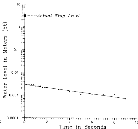
Figure 2. Slug test with atypical (DRR) recovery pattern.
