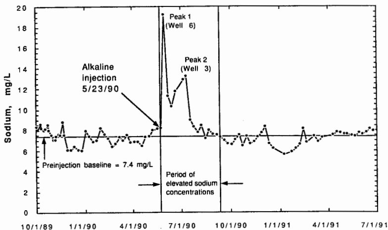
Figure 7. Sodium tracer breakthrough at mine discharge.
