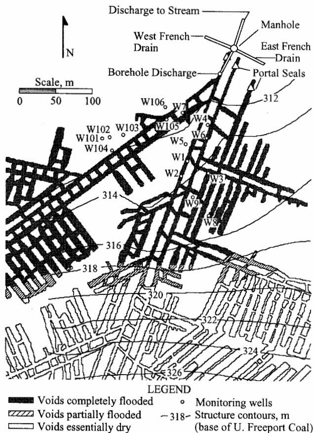
Figure 6. Plan view of underground mine pool study site.
