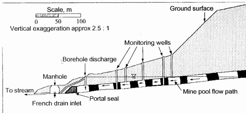
Figure 5. Hypothetical reservoir flow pattern in an underground mine pool
