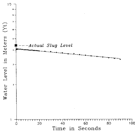
Figure 1. Slug test with typical porous-media recovery pattern.
