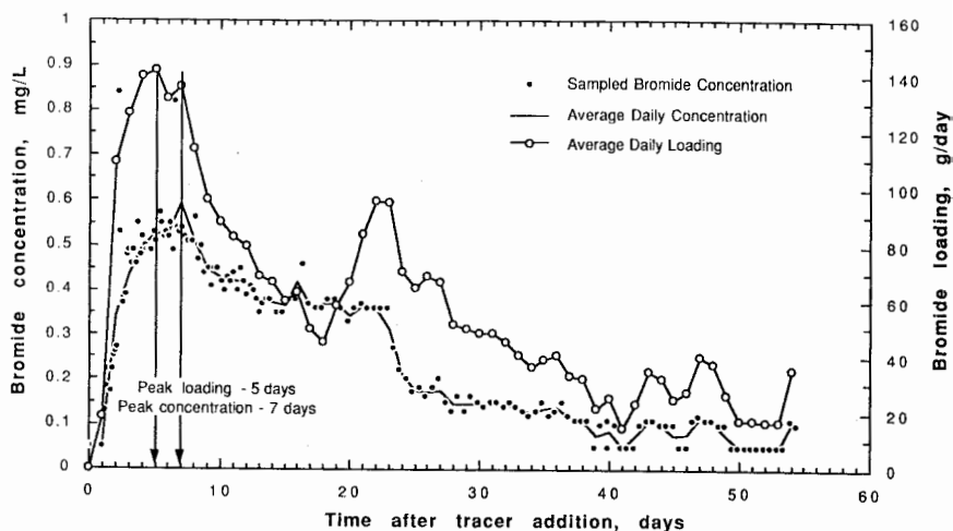
Figure 8. Well 6 bromide tracer test results - manhole outlet.
